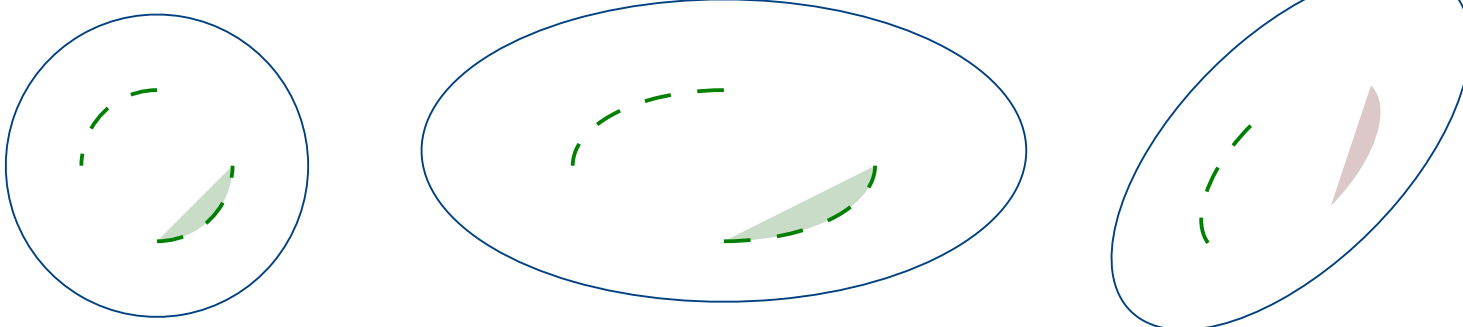
Polygon examples
